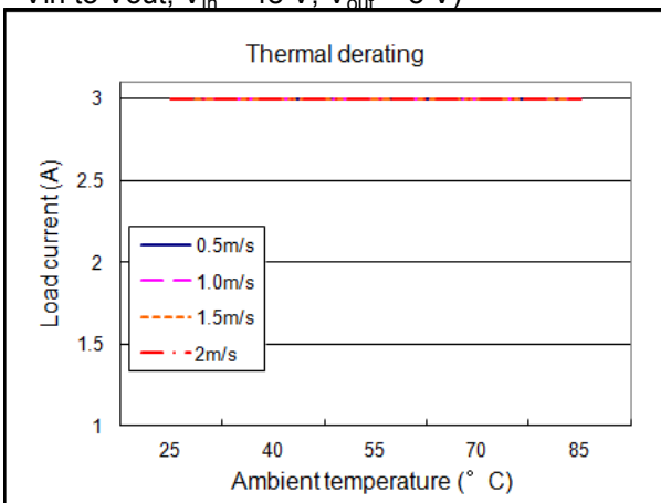
Figure 3: Thermal derating (Air is flowing from Vin to Vout; V_{in} = 48\text{ V} ; V_{out} = 5\text{ V} )
