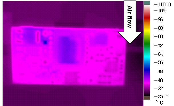
Figure 6: Thermal plot (Air is flowing from Vin(-) to Vin(+); T_A = 25^\circ\text{C} (77°F); Airflow = 1.5 m/s (300 FLM); Vin = 48 V; Vout = 5.0 V; Iout = 3 A)
