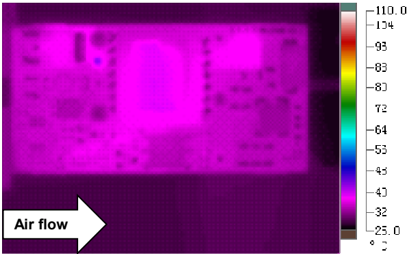
Figure 5: Thermal plot (Air is flowing from Vin to Vout; T_A = 25^\circ\text{C} (77°F); Airflow = 1.5 m/s (300 FLM); Vin = 48 V; Vout = 5.0 V; Iout = 3 A)
