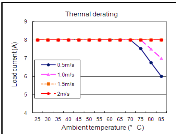
Figure 3: Thermal derating air is flowing from Vin to Vout
