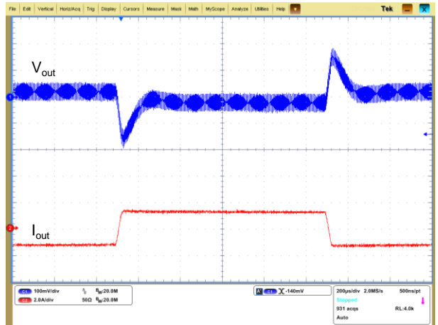
Figure 10: Output voltage response (Load 50%–75%–50%, di/dt=0.1 A/µs)
