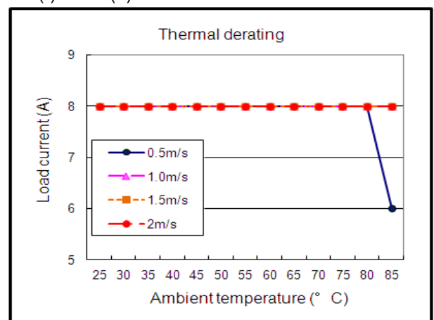
Figure 4: Thermal derating air is flowing from Vin(-) to Vin(+)
