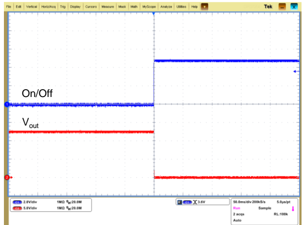
Figure 8: Shutdown from power on
