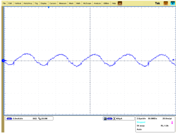
Figure 12: Input reflected ripple current (for point A in the test set-up diagram)
