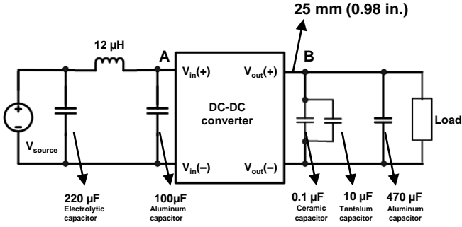
Figure 11: Test set-up diagram
