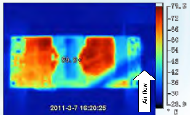
Figure 6: Thermal plot with airflow from V_{in}(-) to V_{in}(+) ( T_A = 25^\circ\text{C} ( 77^\circ\text{F} ); Airflow = 1 m/s (200 FLM); V_{in} = 48\text{ V} ; V_{out} = 3.3\text{ V} ; I_{out} = 15\text{ A} )
