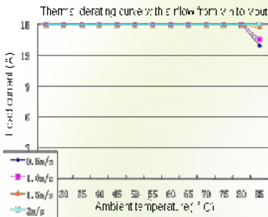
Figure 3: Thermal derating with airflow from V_{in} to V_{out} ( V_{in} = 48\text{ V} ; V_{out} = 3.3\text{ V} )
