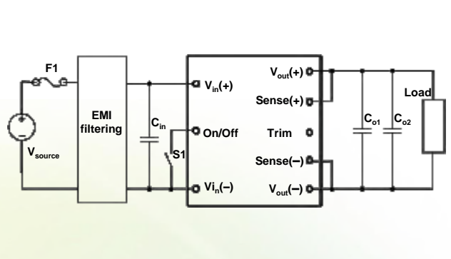
Figure 6: Typical circuit applications
