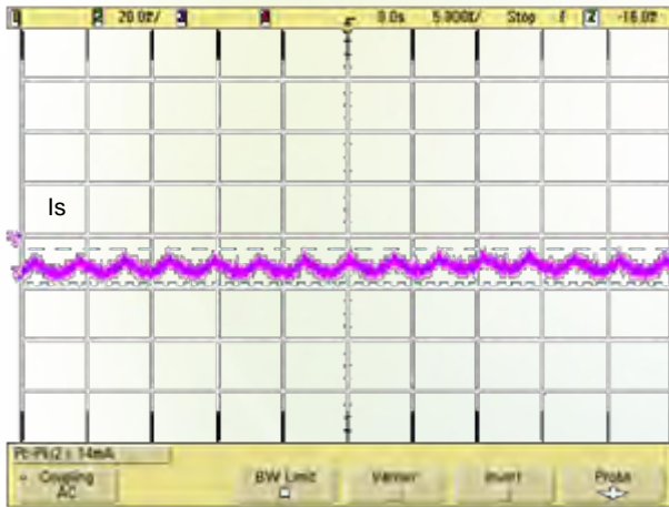
Figure 7: Input reflected ripple current (for point A in the test set-up diagram, V_{\text{in}} = 48\text{ V} , V_{\text{out}} = 48\text{ V} , I_{\text{out}} = 3.2\text{ A} )
