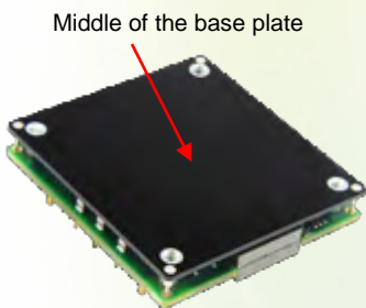
Figure 21: Thermal test point
