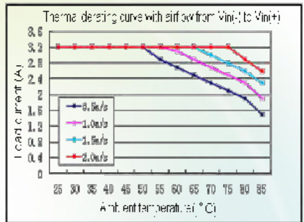
Figure 4: Thermal derating with airflow from V_{in(+)} to V_{in(-)} ( V_{in} = 48\text{ V} ; V_{out} = 48\text{ V} )
