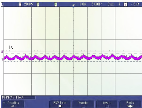
Figure 7: Input reflected ripple current (for point A in the test set-up diagram, V_{\text{in}} = 48\text{ V} , V_{\text{out}} = 53.5\text{ V} , I_{\text{out}} = 1.5\text{ A} )
