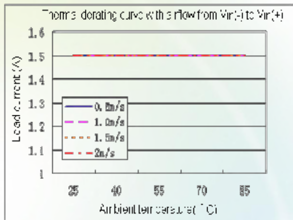
Figure 4: Thermal derating with airflow from V_{in(-)} to V_{in(+)} ( V_{in} = 48\text{ V} ; V_{out} = 53.5\text{ V} )
