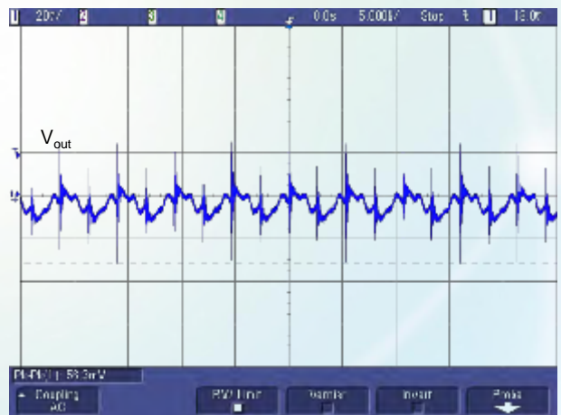
Figure 8: Output voltage ripple (for point B in the test set-up diagram, V_{\text{in}} = 48\text{ V} , V_{\text{out}} = 53.5\text{ V} , I_{\text{out}} = 1.5\text{ A} )
