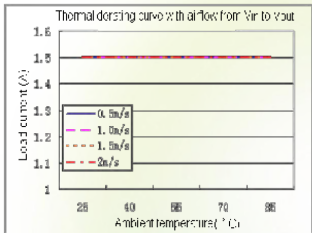
Figure 3: Thermal derating with airflow from V_{in(-)} to V_{out} ( V_{in} = 48\text{ V} ; V_{out} = 53.5\text{ V} )
