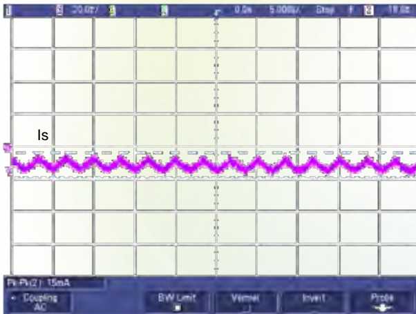
Figure 9: Input reflected ripple current (for point A in the test set-up diagram, V_{\text{in}} = 48\text{ V} , V_{\text{out}} = 12\text{ V} , I_{\text{out}} = 10\text{ A} )
