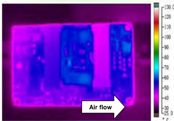
Figure 5: Thermal plot with airflow from V_{in} to V_{out} ( T_A = 25^\circ\text{C} ( 77^\circ\text{F} ); Airflow = 1 m/s (200 FLM); V_{in} = 48\text{ V} ; V_{out} = 12\text{ V} ; I_{out} = 10\text{ A} )
