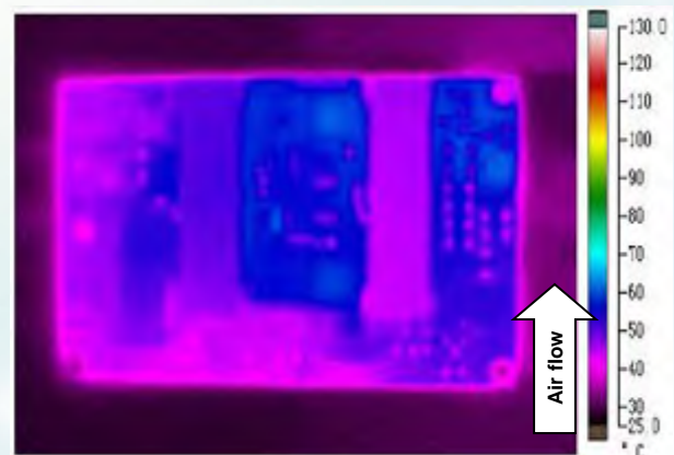
Figure 6: Thermal plot with airflow from V_{in}(-) to V_{in}(+) ( T_A = 25^\circ\text{C} ( 77^\circ\text{F} ); Airflow = 1 m/s (200 FLM); V_{in} = 48\text{ V} ; V_{out} = 12\text{ V} ; I_{out} = 10\text{ A} )
