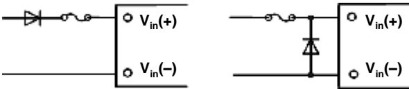
Figure 21: Recommend reverse polarity protection circuits
