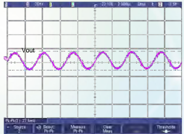
Figure 10: Output voltage ripple (for point B in the test set-up diagram, V_{\text{in}} = 48\text{ V} , V_{\text{out}} = 12\text{ V} , I_{\text{out}} = 10\text{ A} )
