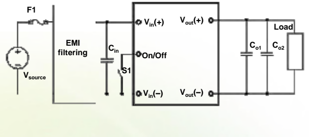
Figure 8: Typical circuit applications
