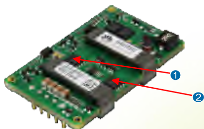
Figure 23: Thermal test point
