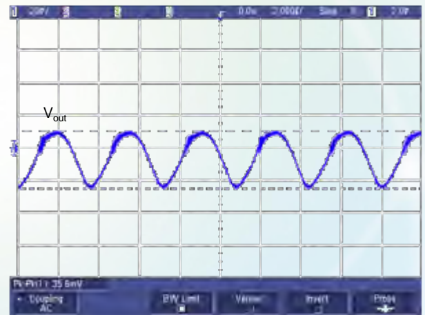
Figure 10: Output voltage ripple (for point B in the test set-up diagram, V_{\text{in}} = 48\text{ V} , V_{\text{out}} = 5\text{ V} , I_{\text{out}} = 20\text{ A} )
