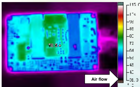
Figure 5: Thermal plot with airflow from V_{in} to V_{out} ( T_A = 25^\circ\text{C} ( 77^\circ\text{F} ); Airflow = 1\text{ m/s} ( 200\text{ FLM} ); V_{in} = 48\text{ V} ; V_{out} = 5\text{ V} ; I_{out} = 20\text{ A} )
