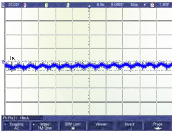
Figure 9: Input reflected ripple current (for point A in the test set-up diagram, V_{\text{in}} = 48\text{ V} , V_{\text{out}} = 5\text{ V} , I_{\text{out}} = 20\text{ A} )
