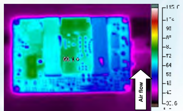
Figure 6: Thermal plot with airflow from V_{in}(-) to V_{in}(+) ( T_A = 25^\circ\text{C} ( 77^\circ\text{F} ); Airflow = 1\text{ m/s} ( 200\text{ FLM} ); V_{in} = 48\text{ V} ; V_{out} = 5\text{ V} ; I_{out} = 20\text{ A} )
