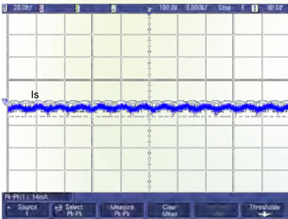
Figure 7: Input reflected ripple current (for point A in the test set-up diagram, V_{\text{in}} = 48\text{ V} , V_{\text{out}} = 3.3\text{ V} , I_{\text{out}} = 25\text{ A} )
