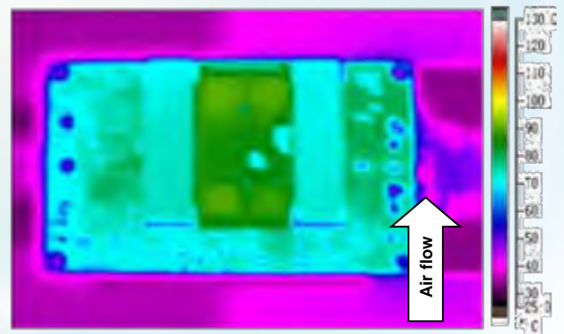
Figure 6: Thermal plot with airflow from V_{in(-)} to V_{in(+)} ( T_A = 25^\circ\text{C} ( 77^\circ\text{F} ); Airflow = 1 m/s (200 FLM); V_{in} = 48\text{ V} ; V_{out} = 1.2\text{ V} ; I_{out} = 30\text{ A} )
