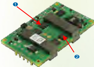
Figure 23: Thermal test point
