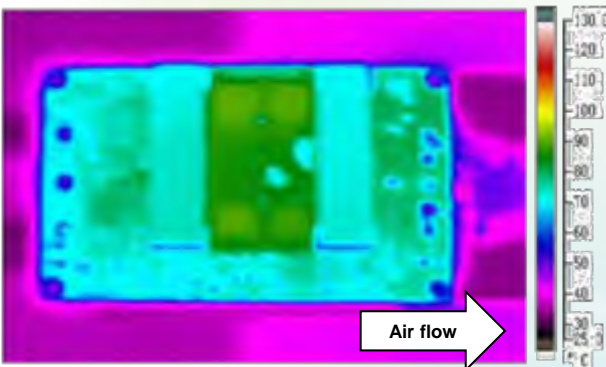
Figure 5: Thermal plot with airflow from V_{in} to V_{out} ( T_A = 25^\circ\text{C} ( 77^\circ\text{F} ); Airflow = 1 m/s (200 FLM); V_{in} = 48\text{ V} ; V_{out} = 1.2\text{ V} ; I_{out} = 30\text{ A} )
