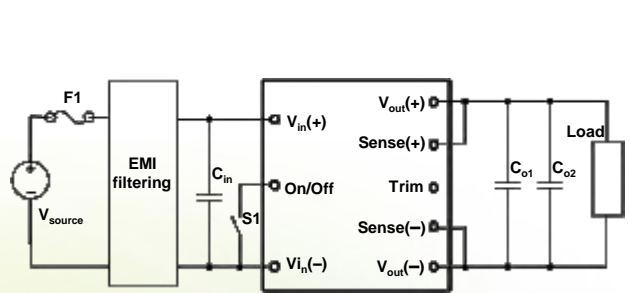
Figure 8: Typical circuit applications
