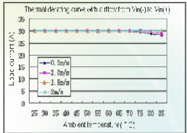
Figure 4: Thermal derating with airflow from V_{in(-)} to V_{in(+)} ( V_{in} = 48\text{ V} ; V_{out} = 1.2\text{ V} )
