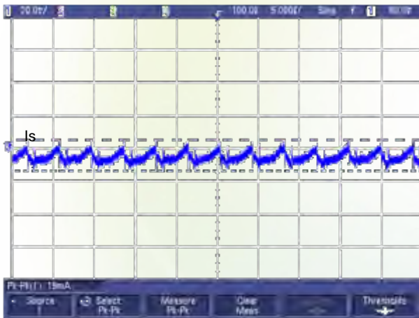
Figure 9: Input reflected ripple current (for point A in the test set-up diagram, V_{\text{in}} = 48\text{ V} , V_{\text{out}} = 1.2\text{ V} , I_{\text{out}} = 30\text{ A} )
