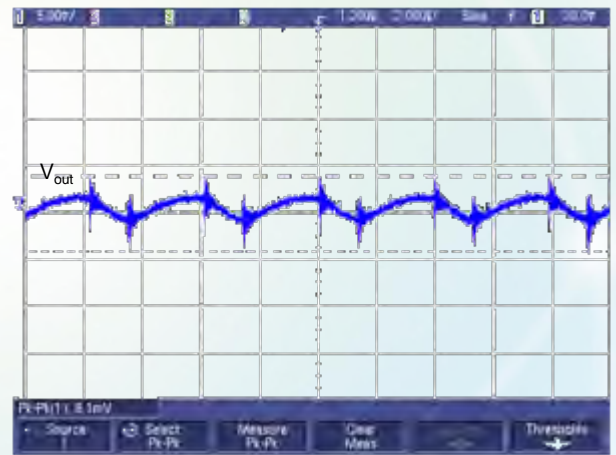
Figure 10: Output voltage ripple (for point B in the test set-up diagram, V_{\text{in}} = 48\text{ V} , V_{\text{out}} = 1.2\text{ V} , I_{\text{out}} = 30\text{ A} )
