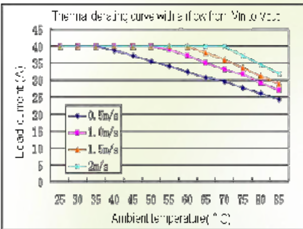
Figure 3: Thermal derating with airflow from V_{in} to V_{out} ( V_{in} = 48\text{ V} ; V_{out} = 1.5\text{ V} )
