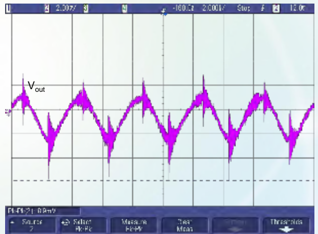
Figure 10: Output voltage ripple (for point B in the test set-up diagram, V_{\text{in}} = 48\text{ V} , V_{\text{out}} = 1.5\text{ V} , I_{\text{out}} = 40\text{ A} )
