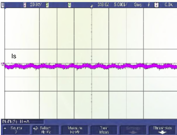
Figure 9: Input reflected ripple current (for point A in the test set-up diagram, V_{\text{in}} = 48\text{ V} , V_{\text{out}} = 1.5\text{ V} , I_{\text{out}} = 40\text{ A} )
