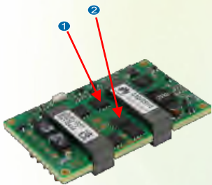
Figure 23: Thermal test point
