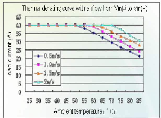
Figure 4: Thermal derating with airflow from V_{in}(+) to V_{in}(-) ( V_{in} = 48\text{ V} ; V_{out} = 1.5\text{ V} )
