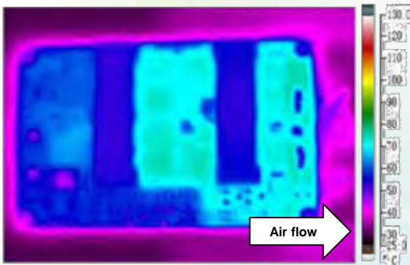
Figure 5: Thermal plot with airflow from V_{in} to V_{out} ( T_A = 25^\circ\text{C} ( 77^\circ\text{F} ); Airflow = 1\text{ m/s} ( 200\text{ FLM} ); V_{in} = 48\text{ V} ; V_{out} = 1.5\text{ V} ; I_{out} = 40\text{ A} )
