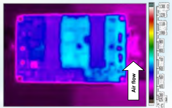
Figure 6: Thermal plot with airflow from V_{in}(+) to V_{in}(-) ( T_A = 25^\circ\text{C} ( 77^\circ\text{F} ); Airflow = 1\text{ m/s} ( 200\text{ FLM} ); V_{in} = 48\text{ V} ; V_{out} = 1.5\text{ V} ; I_{out} = 40\text{ A} )
