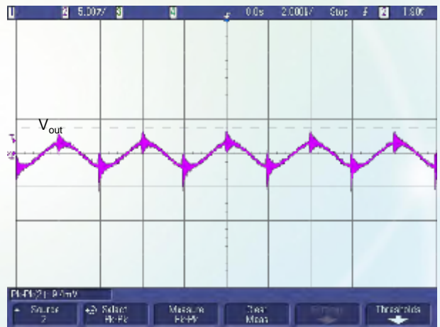
Figure 10: Output voltage ripple (for point B in the test set-up diagram, V_{\text{in}} = 48\text{ V} , V_{\text{out}} = 1.8\text{ V} , I_{\text{out}} = 40\text{ A} )
