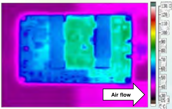
Figure 5: Thermal plot with airflow from V_{in} to V_{out} ( T_A = 25^\circ\text{C} ( 77^\circ\text{F} ); Airflow = 1 m/s (200 FLM); V_{in} = 48\text{ V} ; V_{out} = 1.8\text{ V} ; I_{out} = 40\text{ A} )
