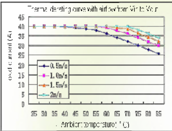
Figure 3: Thermal derating with airflow from V_{in} to V_{out} ( V_{in} = 48\text{ V} ; V_{out} = 1.8\text{ V} )
