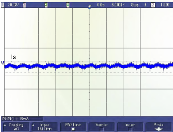
Figure 9: Input reflected ripple current (for point A in the test set-up diagram, V_{\text{in}} = 48\text{ V} , V_{\text{out}} = 1.8\text{ V} , I_{\text{out}} = 40\text{ A} )
