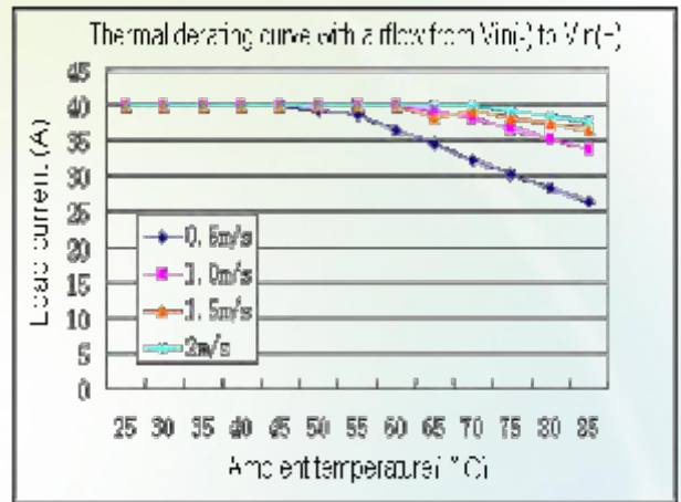
Figure 4: Thermal derating with airflow from V_{in}(-) to V_{in}(+) ( V_{in} = 48\text{ V} ; V_{out} = 1.8\text{ V} )
