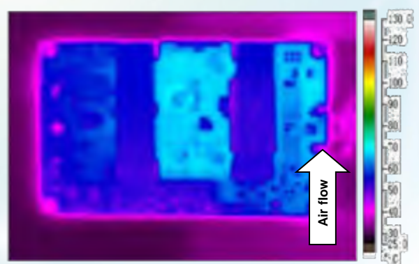
Figure 6: Thermal plot with airflow from V_{in}(-) to V_{in}(+) ( T_A = 25^\circ\text{C} ( 77^\circ\text{F} ); Airflow = 1 m/s (200 FLM); V_{in} = 48\text{ V} ; V_{out} = 1.8\text{ V} ; I_{out} = 40\text{ A} )
