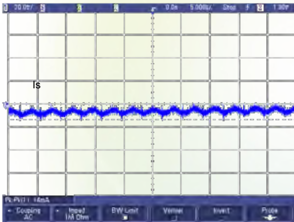
Figure 7: Input reflected ripple current (for point A in the test set-up diagram, V_{\text{in}} = 48\text{ V} ; V_{\text{out}} = 3.3\text{ V} ; I_{\text{out}} = 40\text{ A} )
