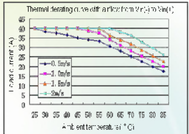
Figure 4: Thermal derating with airflow from V_{in}(-) to V_{in}(+) ( V_{in} = 48\text{ V} ; V_{out} = 3.3\text{ V} )
