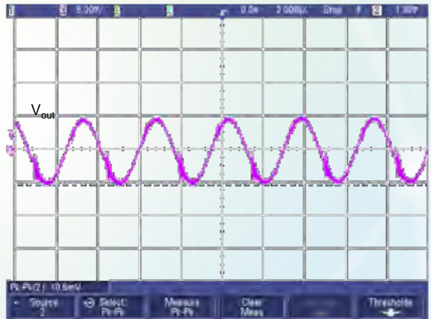
Figure 8: Output voltage ripple (for point B in the test set-up diagram, V_{\text{in}} = 48\text{ V} ; V_{\text{out}} = 3.3\text{ V} ; I_{\text{out}} = 40\text{ A} )
