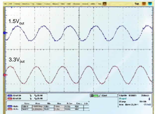
Figure 10: Output voltage ripple (for point BD, CD in the test set-up diagram, V_{in}=48\text{ V} , Output: 3.3 V/8 A, 1.5 V /12 A)
