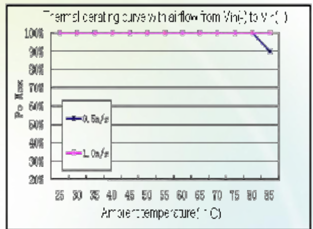
Figure 4: Thermal derating with airflow from V_{in}(-) to V_{in}(+) ( V_{in} = 48\text{ V} ; I_{3.3Vout} and I_{1.5Vout} change synchronous, see erect axis)
