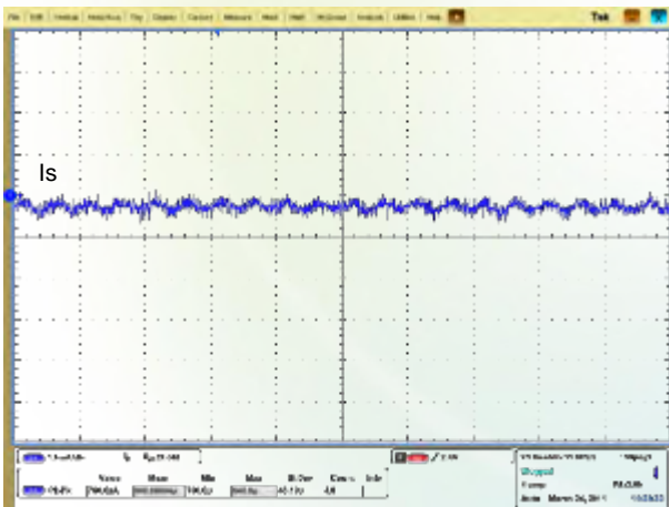
Figure 9: Input reflected ripple current (for point A in the test set-up diagram, V_{in}=48\text{ V} , Output: 3.3 V/8 A, 1.5 V /12 A)
