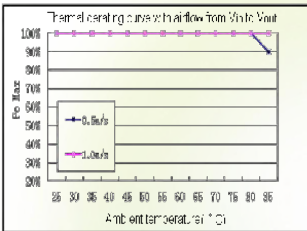
Figure 3: Thermal derating with airflow from V_{in} to V_{out} ( V_{in} = 48\text{ V} ; I_{3.3Vout} and I_{1.5Vout} change synchronous, see erect axis)
