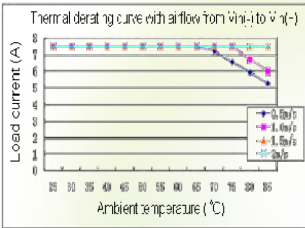
Figure 3: Thermal derating with airflow from V_{in(-)} to V_{in(+)} ( V_{in} = 48\text{ V} ; V_{out} = 12\text{ V} )
