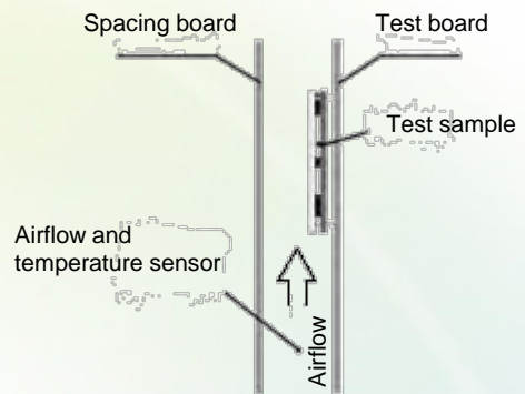
Figure 19: Wind tunnel test setup
