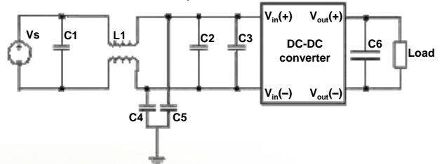
Figure 17: EMC test set-up diagram
