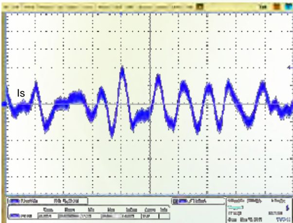
Figure 7: Input reflected ripple current (for point A in the test set-up diagram, V_{\text{in}} = 48\text{ V} , V_{\text{out}} = 12\text{ V} , I_{\text{out}} = 7.5\text{ A} )
