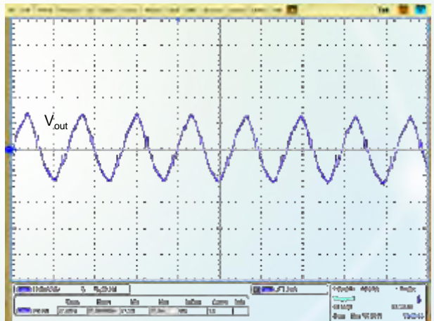
Figure 8: Output voltage ripple (for point B in the test set-up diagram, V_{\text{in}} = 48\text{ V} , V_{\text{out}} = 12\text{ V} , I_{\text{out}} = 7.5\text{ A} )
