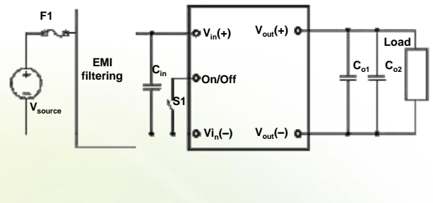
Figure 6: Typical circuit applications
