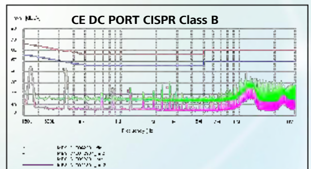
Figure 19: EMC test result
