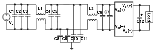
Figure 18: EMC test set-up diagram
