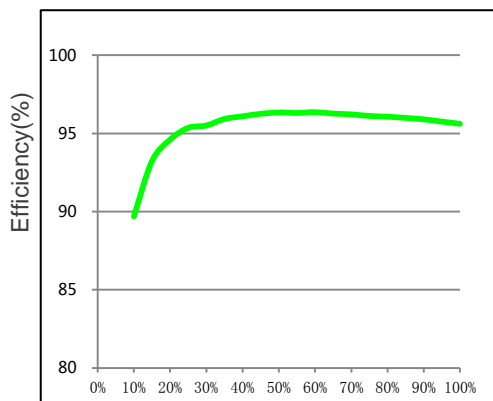
Efficiency curve
