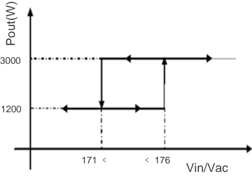
Output power V.S input voltage
